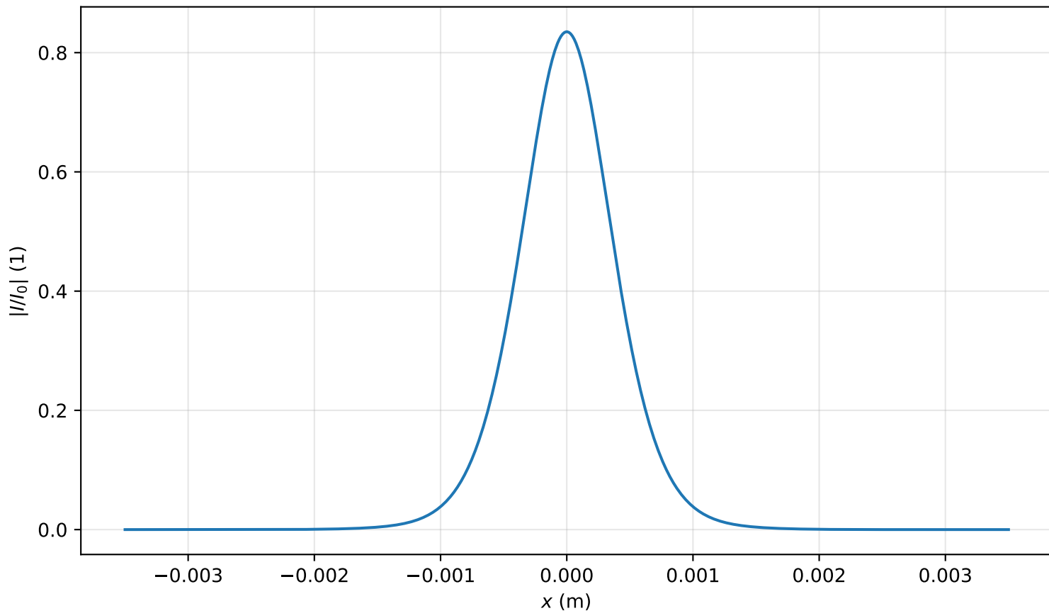
Intensity profile I(x, y = 0, z = 2.388m)/I_0 , P_{in}=0.6P_{cr} , artificial time
